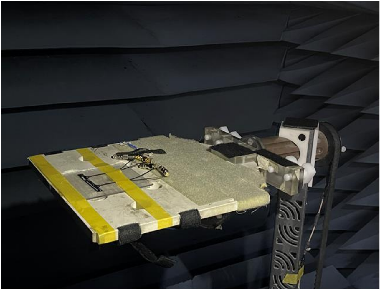
Measurement setup
