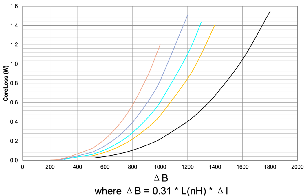
PAL6374.XXXHLT, Core Loss
