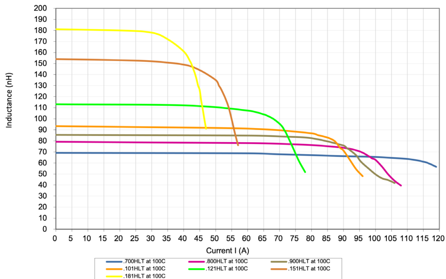
PAL6374.XXXHLT, L vs I, Curve 100°C
