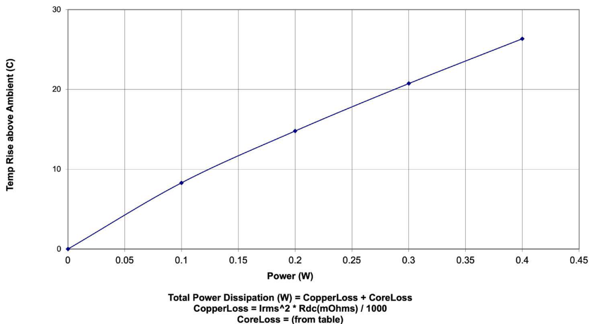
PG2110.XXXHLT Temp Rise vs Power Dissipation
