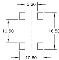
SUGGESTED LAND PATTERN
