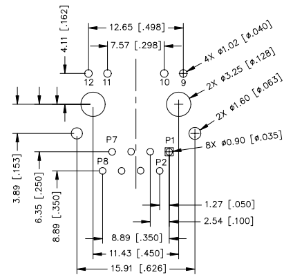
RECOMMENDED PWB LAYOUT (COMPONENT SIDE SHOWN)
