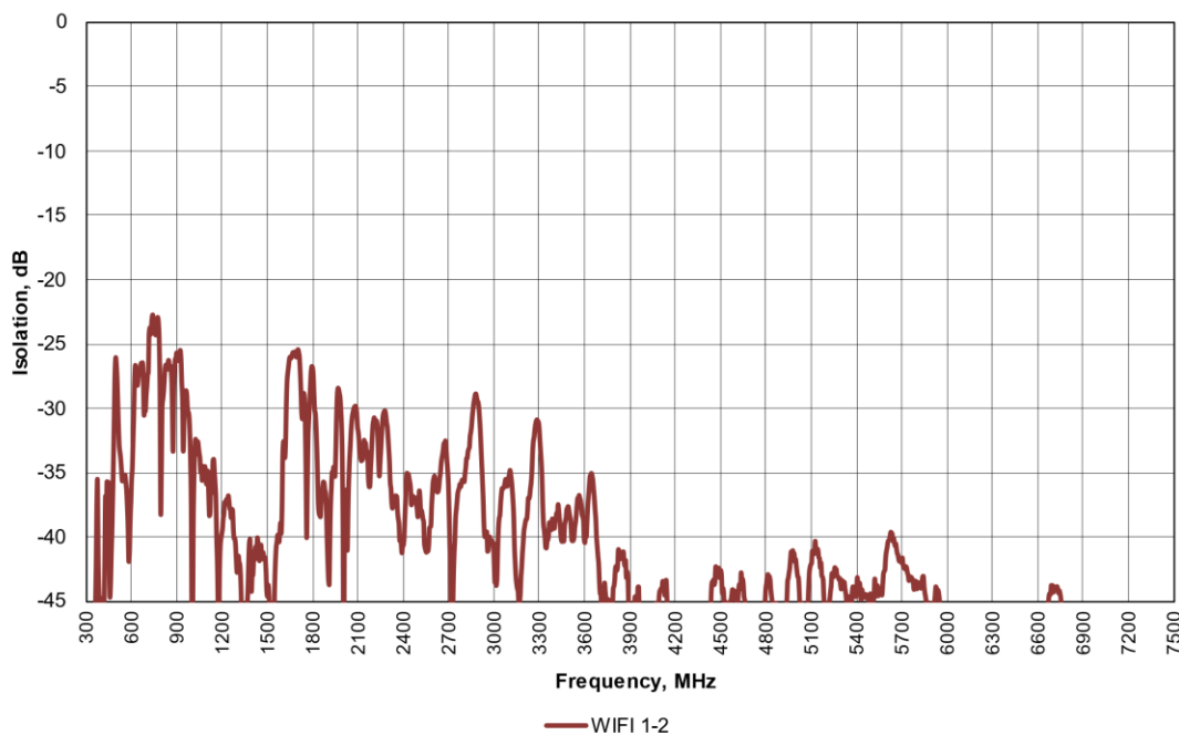
Isolation vs Frequency
