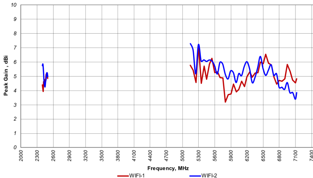
Peak Gain vs Frequency
