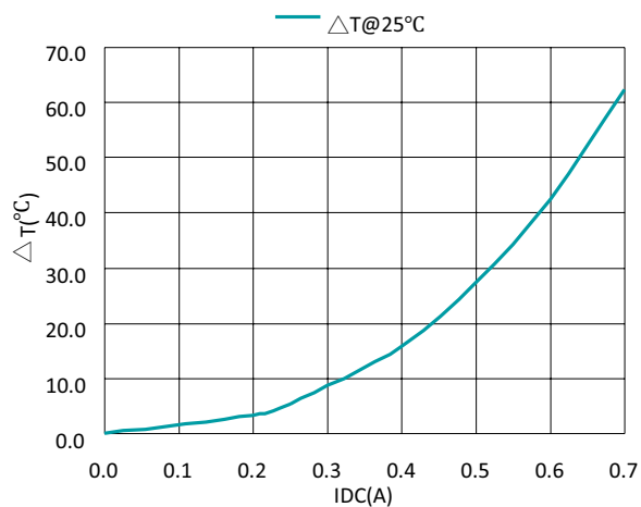
Temp vs DC Current
