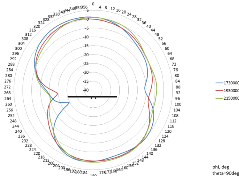
Azimuth plane
