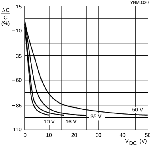
Fig. 4 Typical capacitance change with respect to the capacitance at 1 V as a function of DC voltage at 20 ^{\circ}\text{C}
