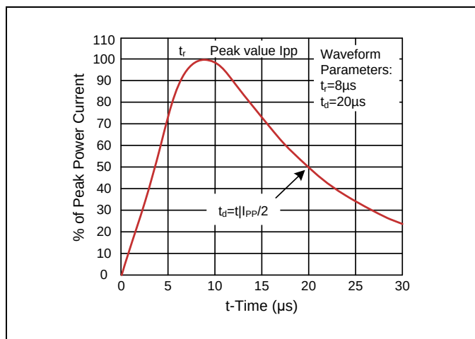
Figure 2. Pulse Waveforms
