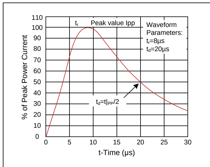
Figure 2. Pulse Waveform
