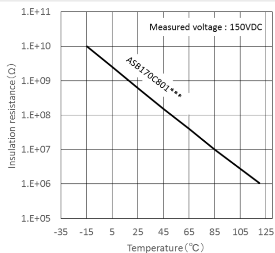
Figure 6 - Temperature vs. Insulation Resistance
