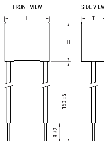
Insulated Flexible Leads 0.5 mm²
