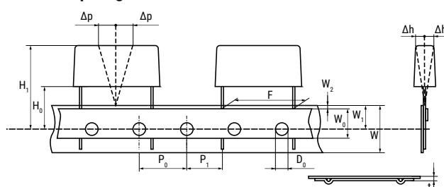
Lead Spacing 22.5 – 27.5 mm
