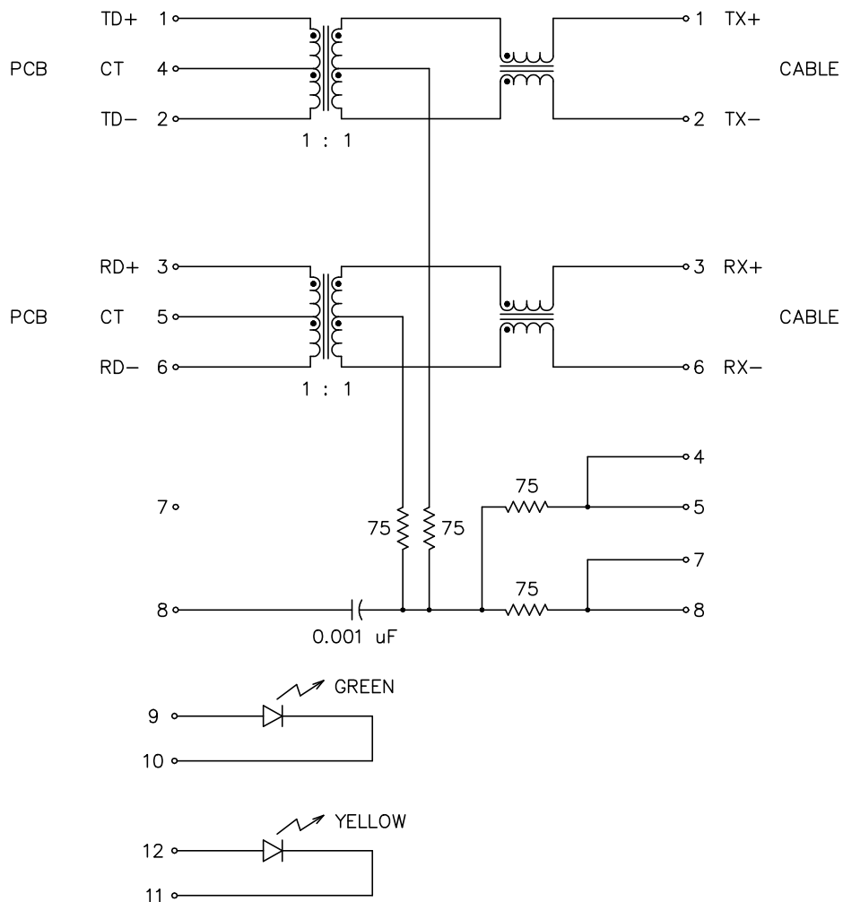
SCHEMATIC
