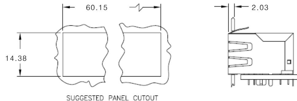
SUGGESTED PANEL CUTOUT
