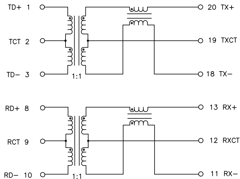
SCHEMATIC
