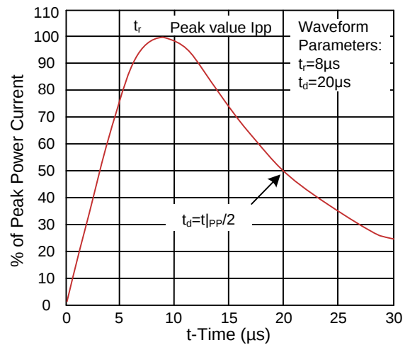
Figure 2. Pulse Waveform
