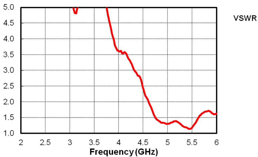
Fig. 3 Return loss & VSWR Measurement
