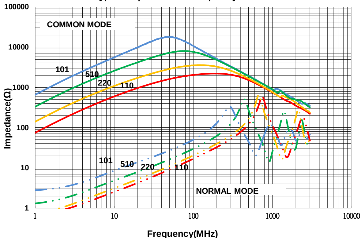
Typical Impedance vs. Frequency Characteristics
