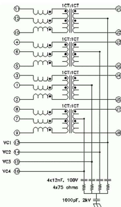
Schematic 1
