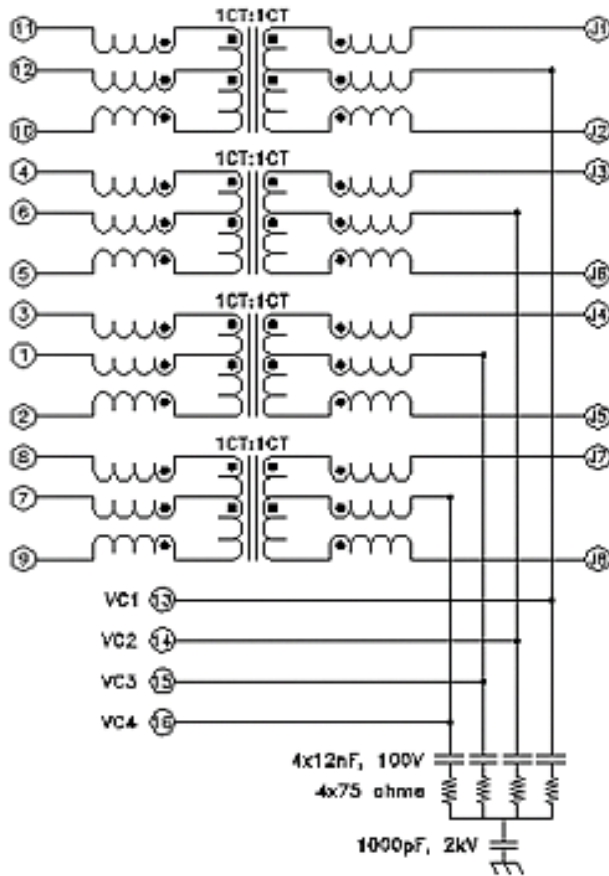
Schematic 4
