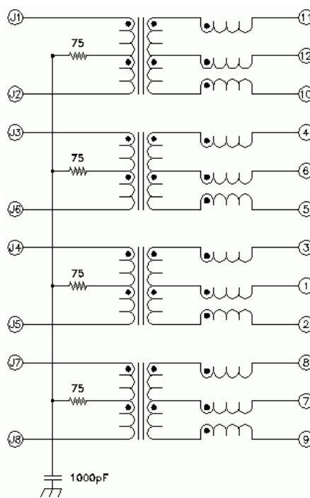
Schematic 2
