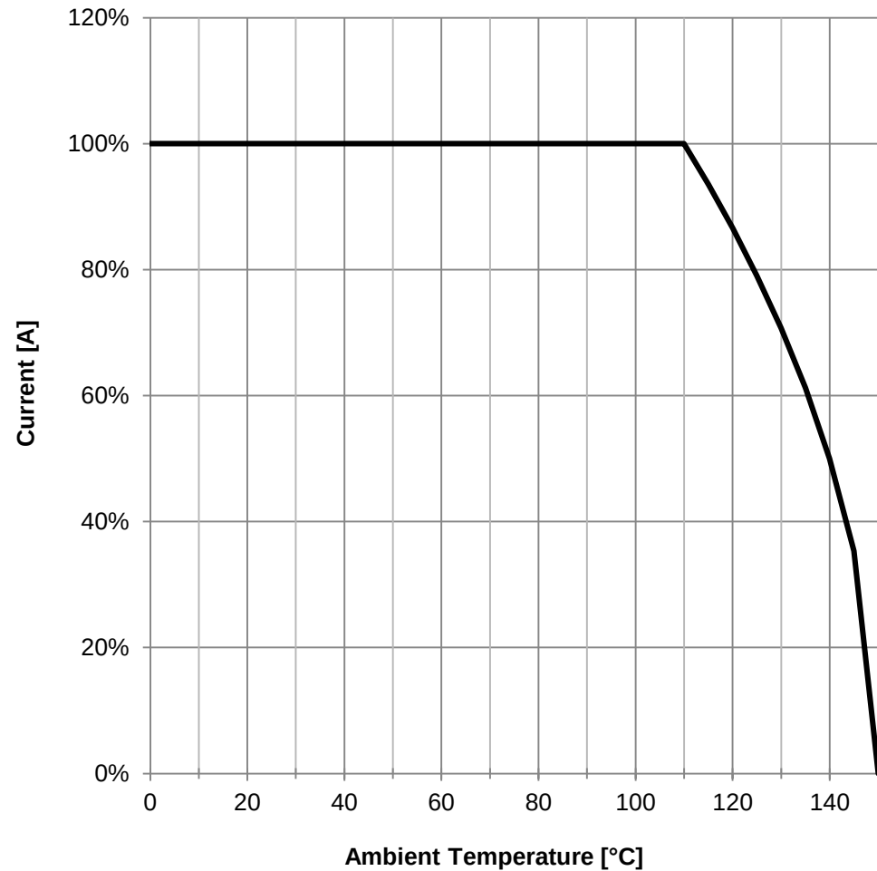
Derating Curve:
