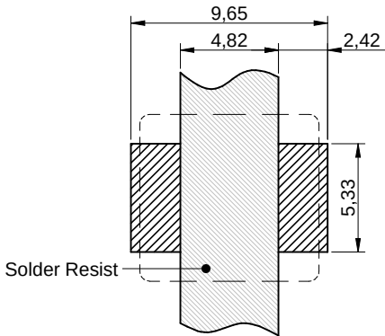
No vias and traces in restricted area. Scale - 2:1
