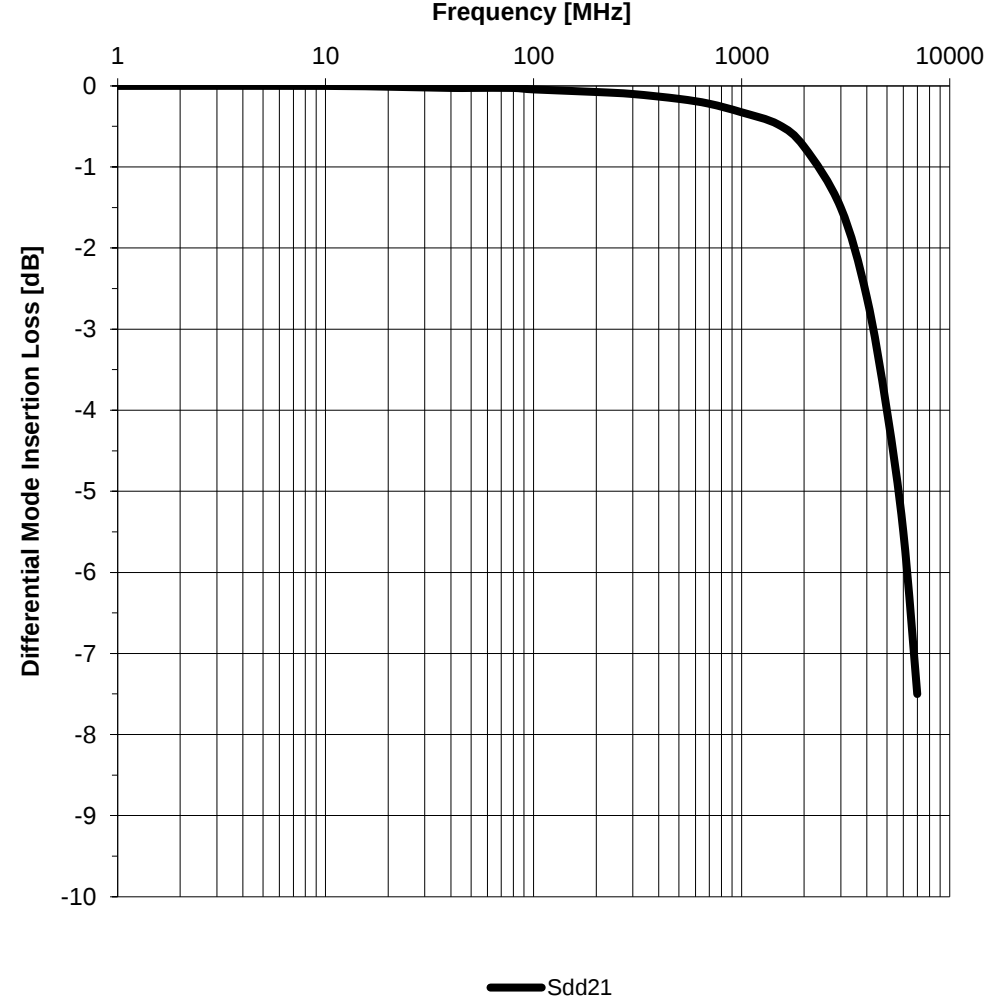
Typical Differential Mode Insertion Loss Characteristics:
