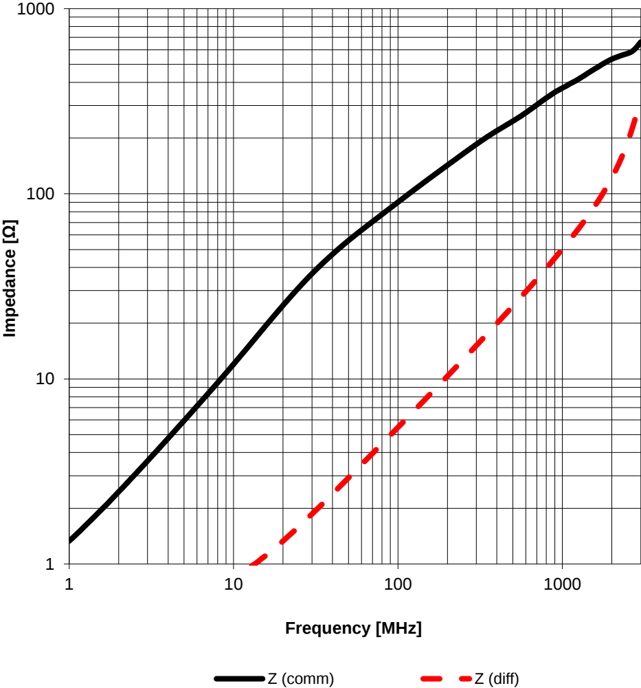
Typical Impedance Characteristics:
