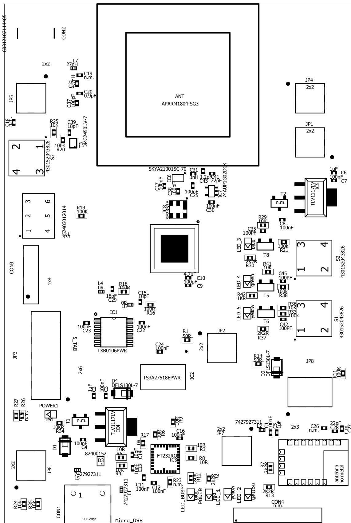
Figure 10: Assembly diagram
