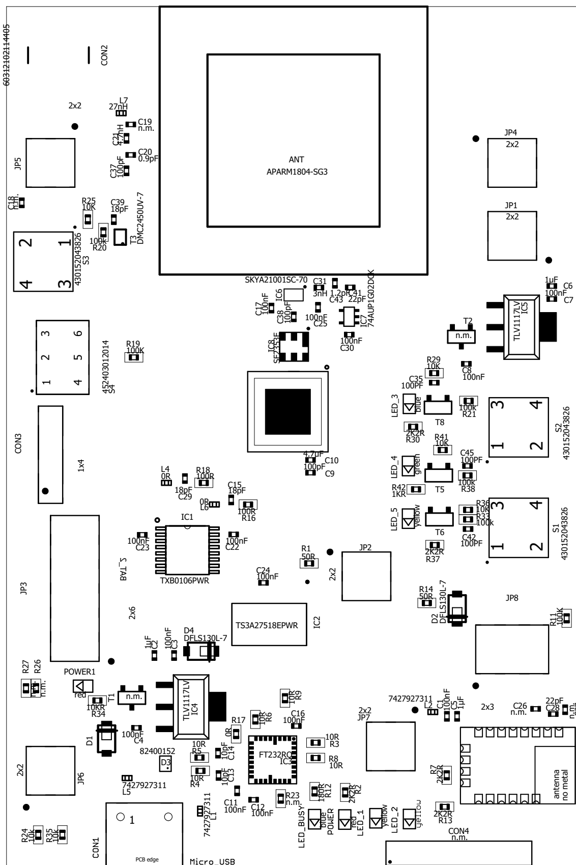
Figure 10: Assembly diagram
