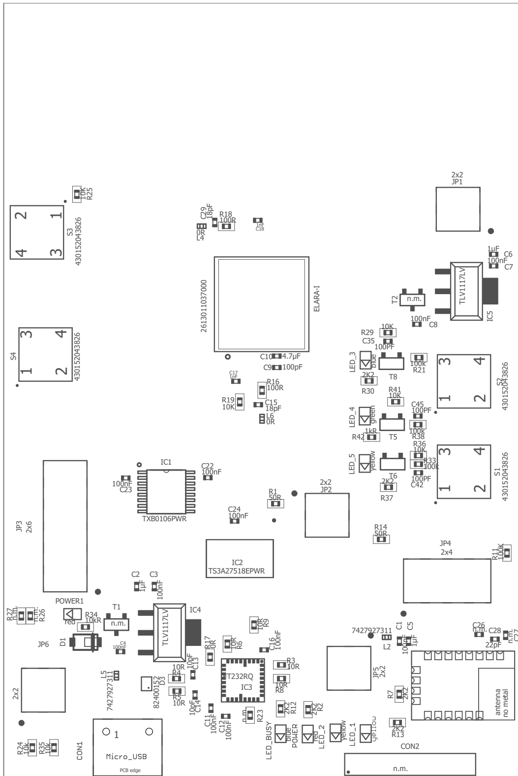
Figure 10: Assembly diagram
