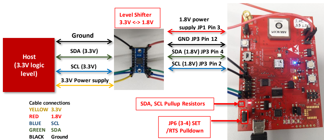
Figure 16: Elara-I- GNSS evaluation board connection to 3.3V Host
