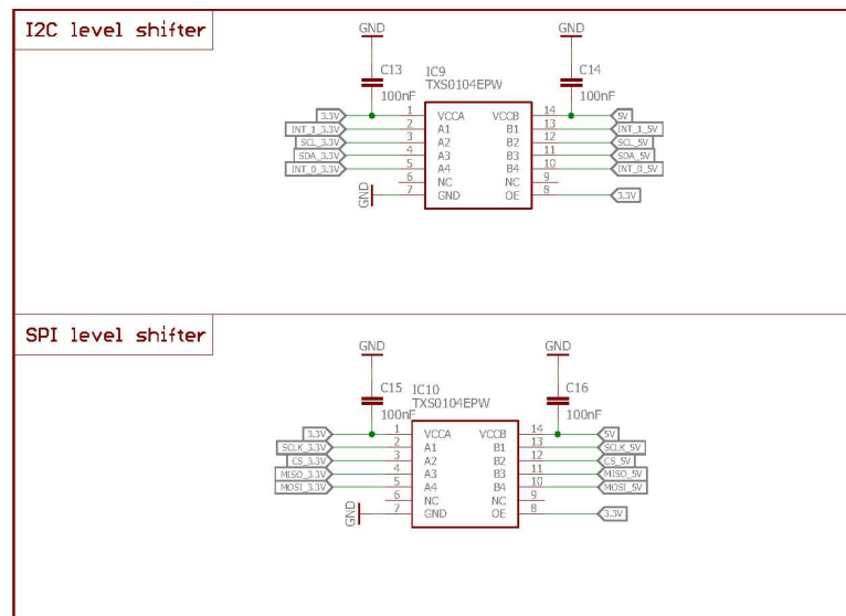
Figure 15: Level shifter
