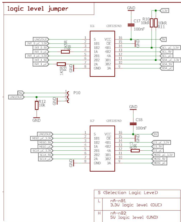
Figure 16: Multiplexer
