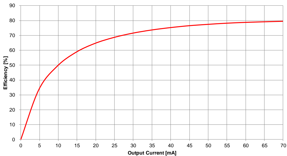
176861512 Efficiency - V_{IN} = 5V , T_A = 25^\circ C
