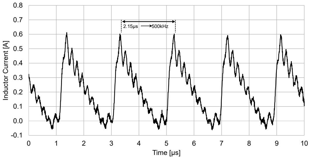
17301xx35 Inductor Ripple Current V_{IN} = 24V , I_{OUT} = 200mA DCM Operation
