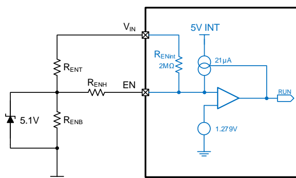
External UVLO circuit with programmable hysteresis and EN pin voltage clamp
