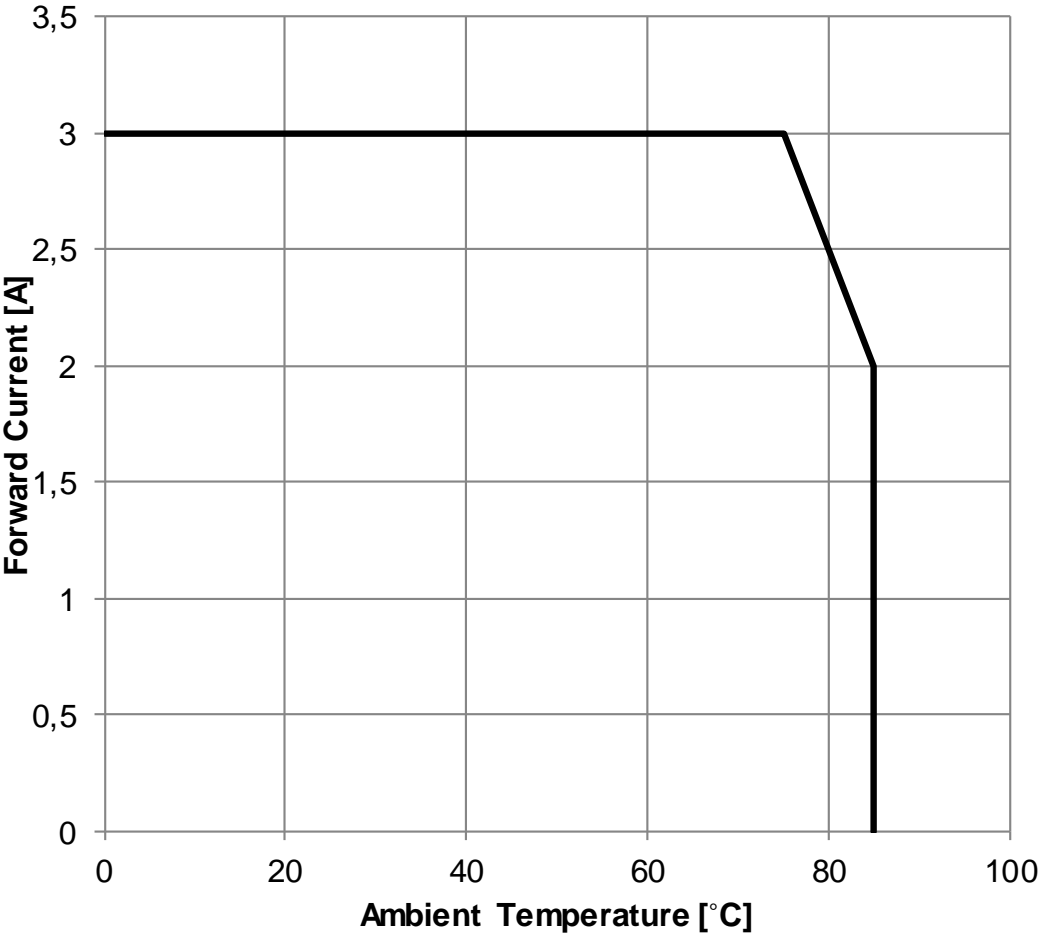
Derating Curve:
