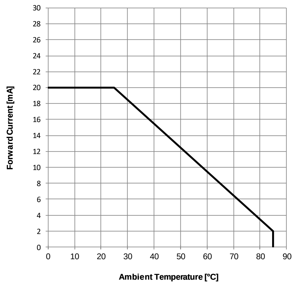
Derating Curve:
