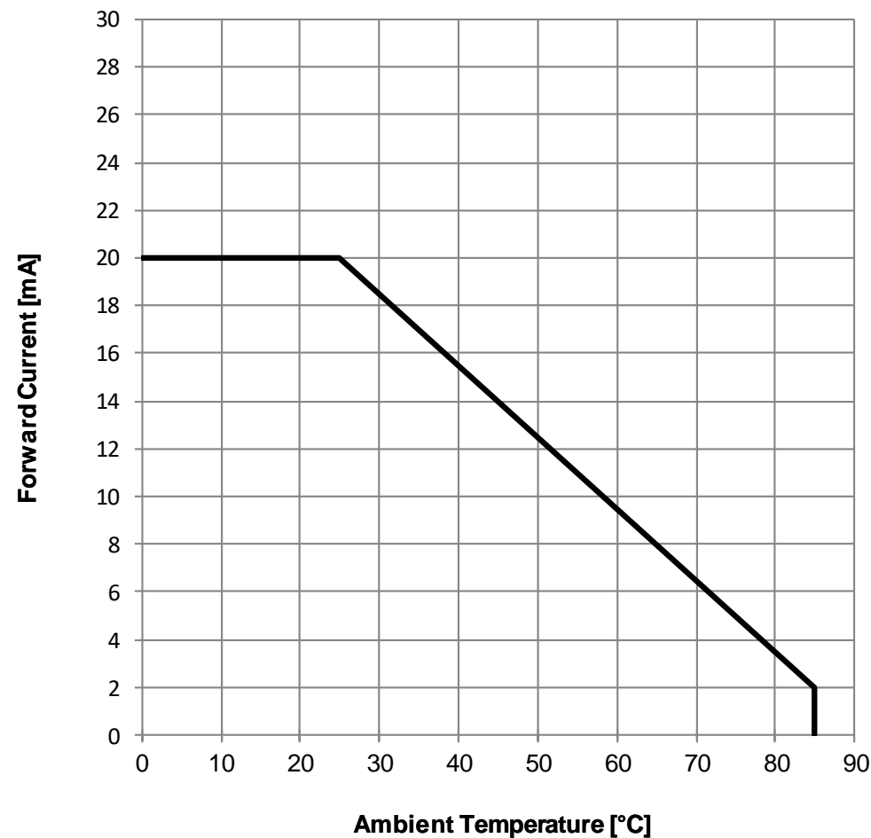
Derating Curve:
