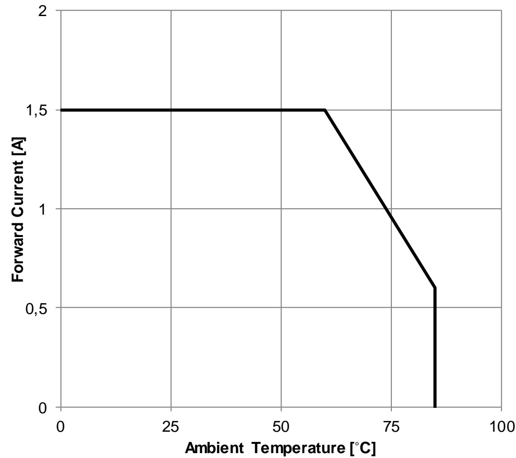
Derating Curve:
