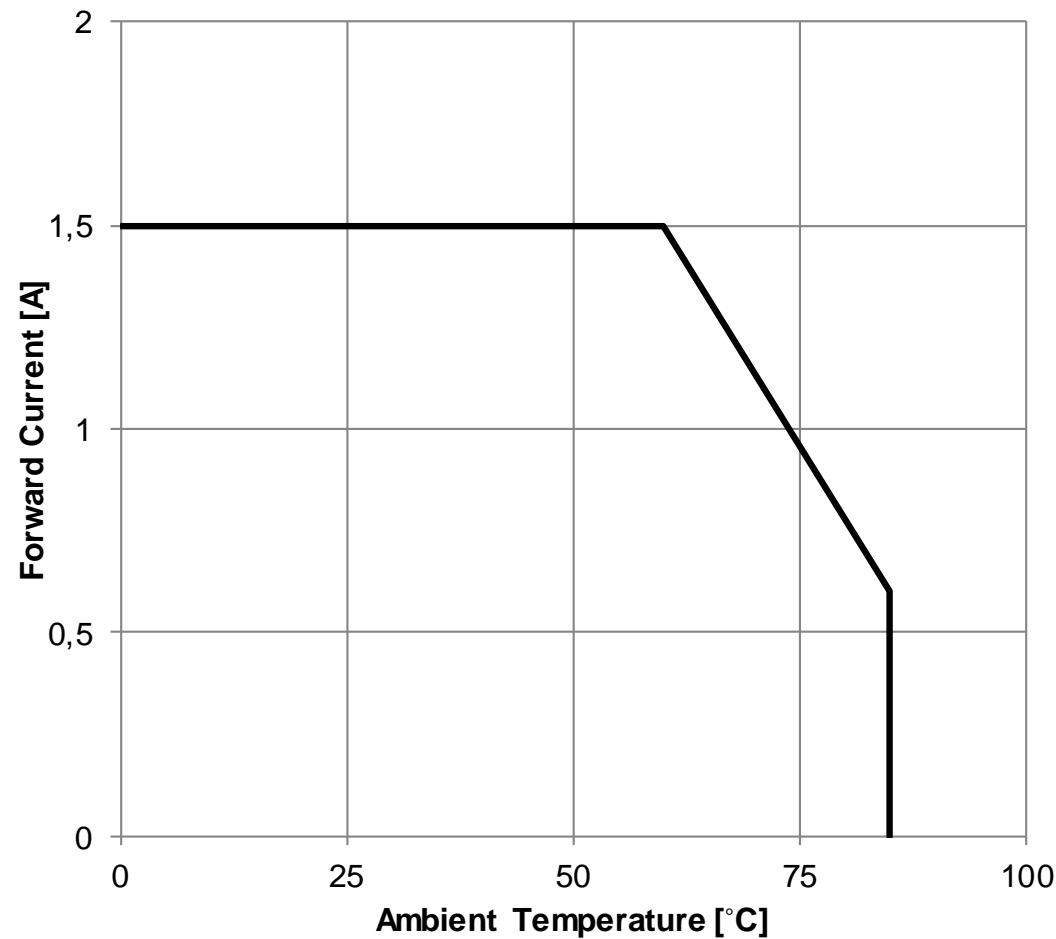
Derating Curve:
