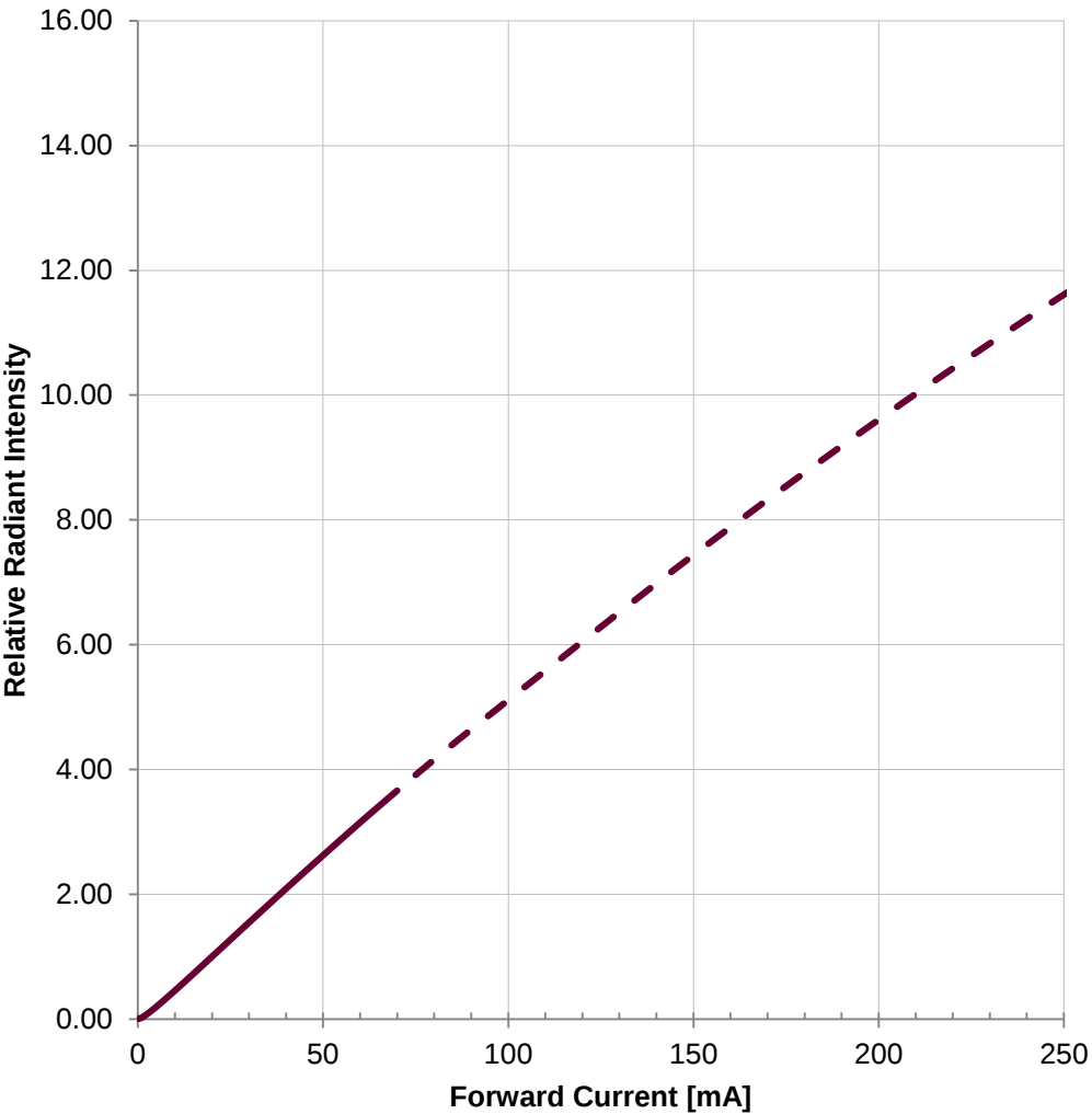
Relative Radiant Intensity vs. Forward Current:
