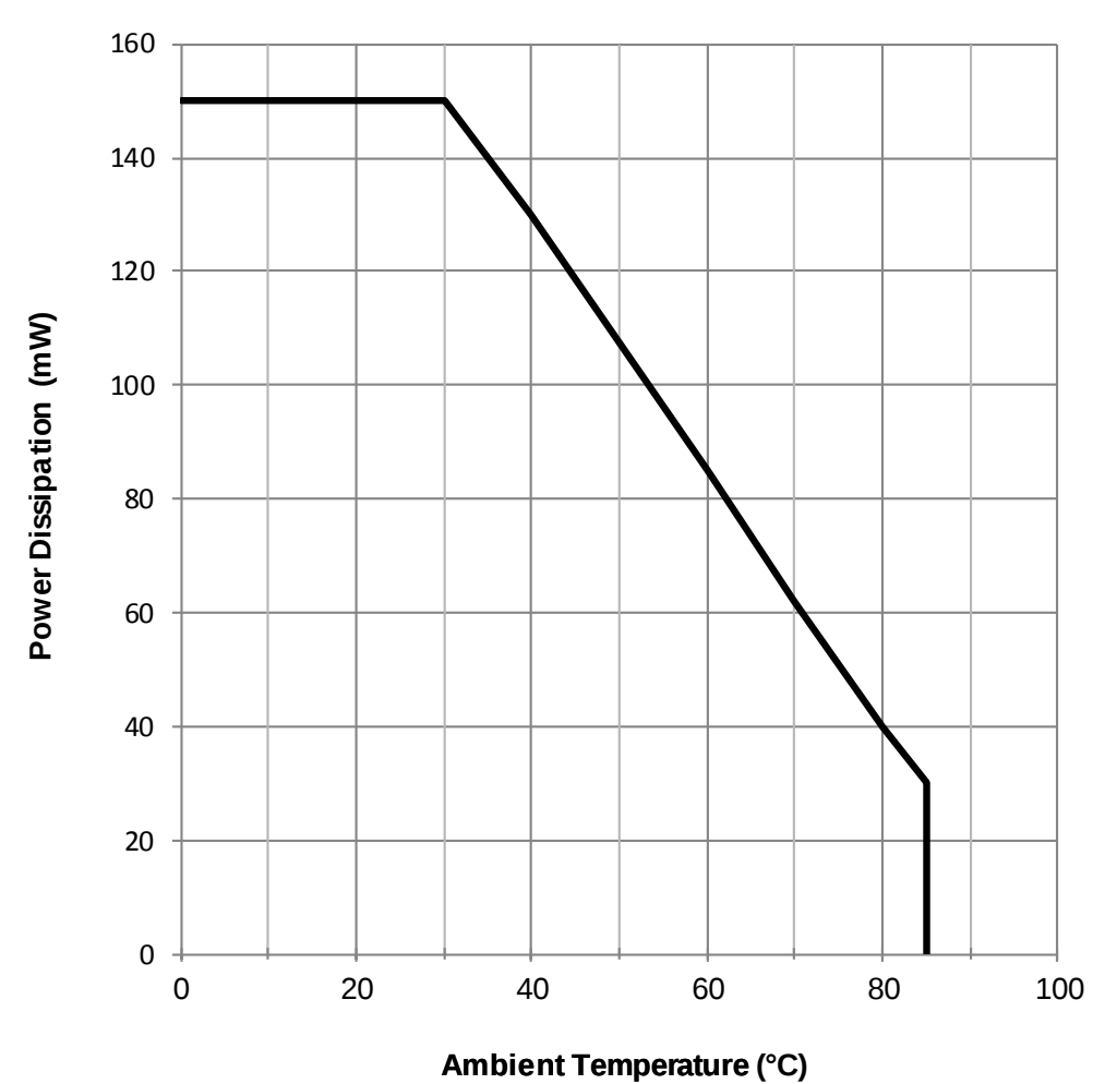
Derating Curve:
