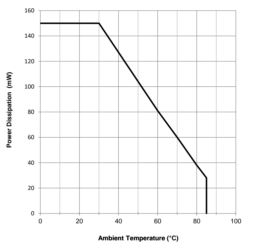
Derating Curve:
