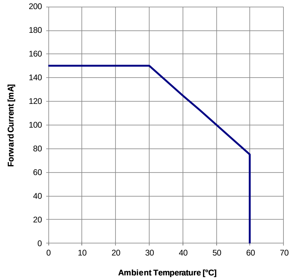
Derating Curve:
