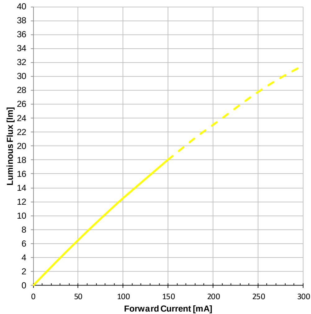
Luminous Flux vs. Forward current:
