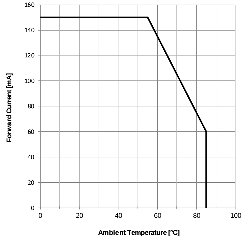
Derating Curve:
