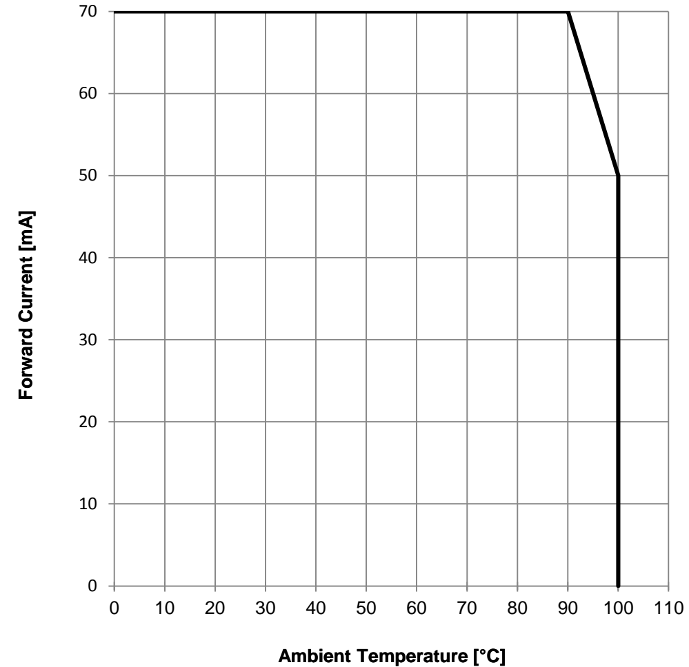
Derating Curve:
