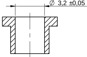
sectional drawing A-A
