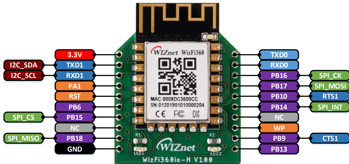
Figure 2. WizFi360io-H Pinout
