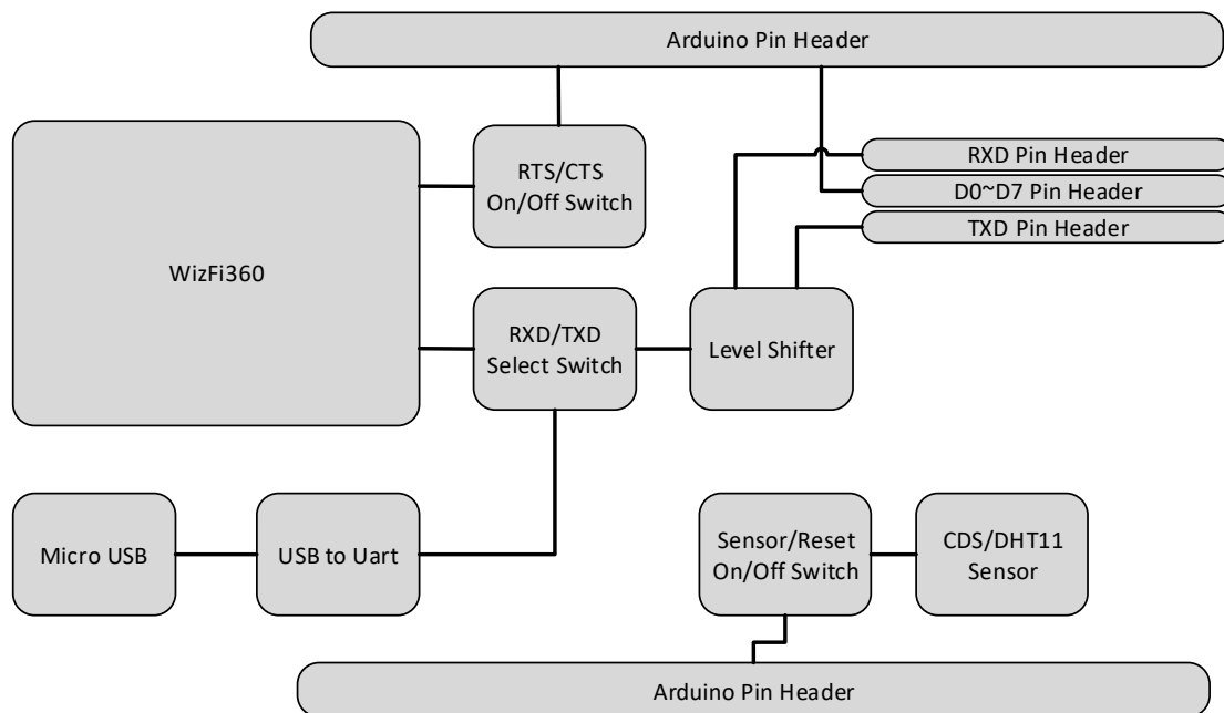
Figure 1. WizFi360-EVB Blockdiagram
