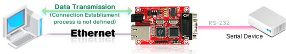
Figure 6. UDP mode
