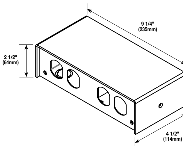
Isoduct® 4-Gang Lab Bench Table Box (AL241S-HB) installed on a work surface.
