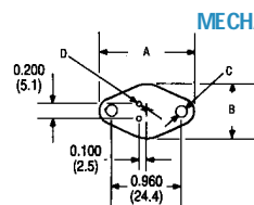
TO-66
