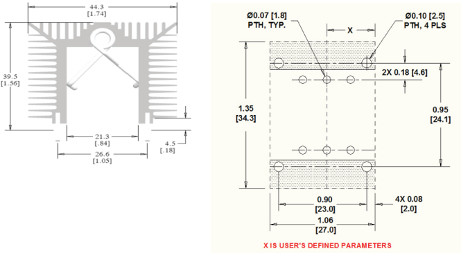
MECHANICAL DIMENSIONS
