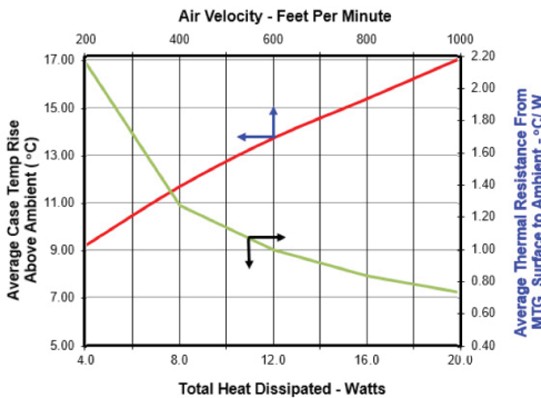
THERMAL RESISTANCE
