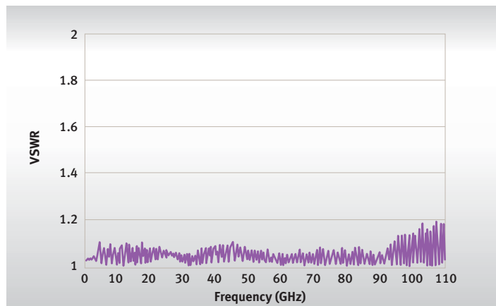
FIGURE 7: TYPICAL VSWR 1
